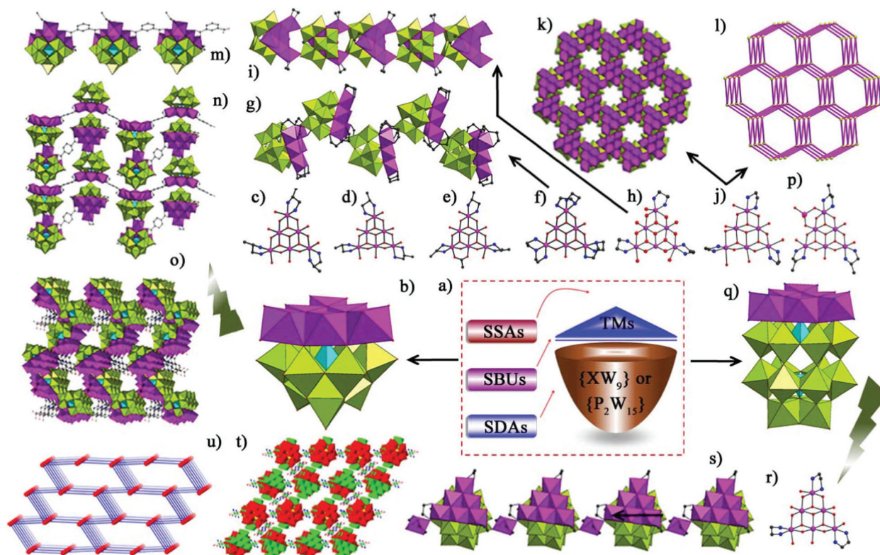
Fig. 2 (a) A schematic synthetic strategy in preparing high-nuclear TMSPTs. (b) View of the \text{TM}_6 -substituted trilacunary Keggin ( \text{TM}_6(\mu_3\text{-OH})_3(\text{H}_2\text{O})_n(\text{L})_3(\text{B-}\alpha\text{-XW}_9\text{O}_{34}) ) monomeric unit. (c, d) View of \text{Ni}_6 -cores in two isomeric units \{\text{Ni}_6(\mu_3\text{-OH})_3(\text{H}_2\text{O})_6(\text{enMe})_3(\text{B-}\alpha\text{-SiW}_9\text{O}_{34})\} . (e) View of the \text{Ni}_6 -core in \{\text{Ni}_6(\mu_3\text{-OH})_3(\text{H}_2\text{O})_4(\text{enMe})_3(\text{CH}_3\text{COO})(\text{B-}\alpha\text{-PW}_9\text{O}_{34})\} . (f, g) View of the \text{Ni}_6 -core in \{\text{Ni}_6(\mu_3\text{-OH})_3(\text{H}_2\text{O})_2(\text{dien})_3(\text{B-}\alpha\text{-PW}_9\text{O}_{34})\} and the 1-D chain structure of [\text{Ni}_6(\mu_3\text{-OH})_3(\text{H}_2\text{O})_2(\text{dien})_3(\text{B-}\alpha\text{-PW}_9\text{O}_{34})]\cdot 4\text{H}_2\text{O} . (h, i) View of the \text{Cu}_6 -core in \{\text{Cu}_6(\mu_3\text{-OH})_3(\text{en})_3(\text{H}_2\text{O})_3(\text{B-}\alpha\text{-PW}_9\text{O}_{34})\} and the 1-D chain structure of [\text{Cu}_6(\mu_3\text{-OH})_3(\text{en})_3(\text{H}_2\text{O})_3(\text{B-}\alpha\text{-PW}_9\text{O}_{34})]\cdot 4\text{H}_2\text{O} . (j) View of the \text{Cu}_6 -core in \{\text{Cu}_6(\mu_3\text{-OH})_3(\text{en})_3(\text{H}_2\text{O})_3(\text{B-}\alpha\text{-PW}_9\text{O}_{34})\} . (k, l) View of the 3-D framework and “Archimedean-type” topology view of [\text{Cu}_6(\mu_3\text{-OH})_3(\text{en})_3(\text{H}_2\text{O})_3(\text{B-}\alpha\text{-PW}_9\text{O}_{34})]\cdot 7\text{H}_2\text{O} [the lime balls are six-connected nodes on behalf of \{\text{Cu}_6(\mu_3\text{-OH})_3(\text{en})_3(\text{H}_2\text{O})_3(\text{B-}\alpha\text{-PW}_9\text{O}_{34})\} units]. (m) The 1-D chain of \{[\text{Ni}_6(\text{OH})_3(\text{H}_2\text{O})_2(\text{enMe})_3(\text{PW}_9\text{O}_{34})](1,3\text{-bdc})\}[\text{Ni}(\text{enMe})_2]\cdot 4\text{H}_2\text{O} . (n) View of the 2-D layer of \{[\text{Ni}_6(\text{OH})_3(\text{H}_2\text{O})(\text{en})_3(\text{PW}_9\text{O}_{34})][\text{Ni}_6(\text{OH})_3(\text{H}_2\text{O})_4(\text{en})_3(\text{PW}_9\text{O}_{34})](1,4\text{-bdc})_{1.5}\}[\text{Ni}(\text{en})(\text{H}_2\text{O})_4]\cdot \text{H}_2\text{O} . (o) The 3-D architecture of \{[\text{Ni}_6(\text{OH})_3(\text{H}_2\text{O})_5(\text{PW}_9\text{O}_{34})](1,2,4\text{-Hbct})\}\cdot \text{H}_2\text{enMe}\cdot 5\text{H}_2\text{O} . (p) View of the \text{Ni}_7 -core in \{[\text{Ni}_7(\mu_3\text{-OH})_3\text{O}_2(\text{dap})_3(\text{H}_2\text{O})_6(\text{B-}\alpha\text{-PW}_9\text{O}_{34})]\} . (q) View of the \text{TM}_6 -substituted trilacunary Dawson ( \text{TM}_6(\mu_3\text{-OH})_3(\alpha\text{-P}_2\text{W}_{15}\text{O}_{56}) ) monomeric unit. (r, s) View of the \text{Ni}_6 -core in \{\text{Ni}_6(\mu_3\text{-OH})_3(\text{H}_2\text{O})_6(\text{en})_3\text{H}(\alpha\text{-P}_2\text{W}_{15}\text{O}_{56})\} and the 1-D chain structure of [\text{Ni}(\text{en})_2][\text{Ni}_6(\mu_3\text{-OH})_3(\text{H}_2\text{O})_6(\text{en})_3\text{H}(\alpha\text{-P}_2\text{W}_{15}\text{O}_{56})]\cdot 5.5\text{H}_2\text{O} . (t, u) View of the 3-D framework and the \text{SrAl}_2 topology of [\text{Ni}(\text{enMe})_2]_3[\text{Ni}(\text{enMe})_2(\text{H}_2\text{O})][\text{Ni}(\text{enMe})(\text{H}_2\text{O})_2][\text{Ni}_6(\text{enMe})_3(\mu_3\text{-OH})_3(\text{Ac})_2(\text{H}_2\text{O})(\text{P}_2\text{W}_{15}\text{O}_{56})]_2\cdot 6\text{H}_2\text{O} . [Copied from ref. 14b]. \{\text{WO}_6\} : lime, \{\text{XO}_4\} : turquoise, TM and \{\text{TMO}_x\text{N}_y\} : light lavender, O: red, C: cray-80%, N: blue]. (t) and (u) are reprinted with permission from ref. 14b. Copyright 2014 Wiley-VCH Verlag GmbH & Co. KGaA, Weinheim.
