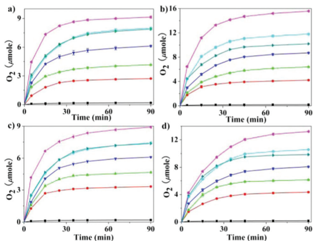
Fig. 20 (a–d) Kinetics of O_2 evolution in the photocatalytic system at different concentrations of Co_{14} -ST, Co_{14} -GT, Co_{14} -PT and Co_{14} -AT. [Concentrations: 0 \mu M , 3 \mu M , 5 \mu M , 10 \mu M , 15 \mu M , 20 \mu M , 30 \mu M . Conditions: 300 W Xe lamp, 420–800 nm; 1.0 mM [Ru(bpy)_3]Cl_2 , 5.0 mM Na_2S_2O_8 , sodium borate buffer pH 9.0 (80 mM); total reaction volume 20 mL; vigorous stirring ( 1.5 \times 10^3 rpm)] [Fig. 21a–d is reprinted with permission from ref. 38a. Copyright 2014 American Chemical Society].
