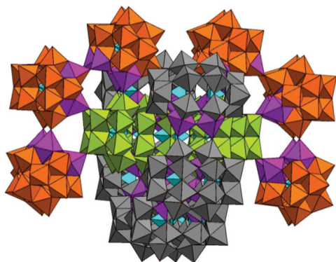
Fig. 16 The core-shell cluster architecture of [(\text{P}_8\text{W}_{48}\text{O}_{184})\{(\text{P}_2\text{W}_{14}\text{Mn}_4\text{O}_{60})(\text{P}_2\text{W}_{15}\text{Mn}_3\text{O}_{58})_2\}_4]^{144-} . \{\text{WO}_6\} in tri-Dawson PT subunits \{(\text{P}_2\text{W}_{14}\text{Mn}_4\text{O}_{60})(\text{P}_2\text{W}_{15}\text{Mn}_3\text{O}_{58})_2\} : lime or gray-50%, \{\text{WO}_6\} in the \{\text{P}_8\text{W}_{48}\text{O}_{184}\} wheel: orange, \{\text{PO}_4\} : turquoise, \{\text{MnO}_6\} : light lavender, O: red.
