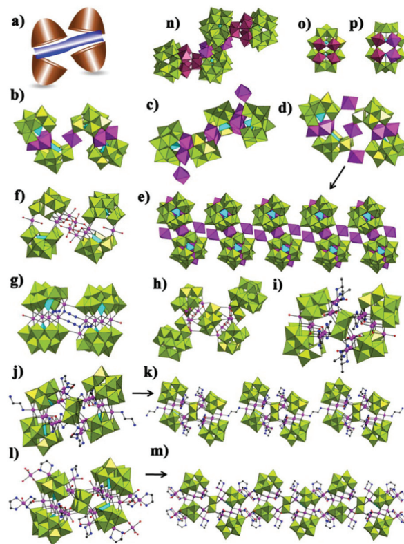
Fig. 9 (a) The schematic mode of “S”-shaped TMSPTs. (b) View of [(\text{B}-\beta\text{-SiW}_9\text{O}_{33}(\text{OH}))(\beta\text{-SiW}_8\text{O}_{29}(\text{OH})_2)\text{Co}_3(\text{H}_2\text{O})_2]_2\text{Co}(\text{H}_2\text{O})_2]^{20-} . (c) View of [\text{Mn}_2^{\text{II}}(\text{Mn}^{\text{III}}(\text{H}_2\text{O})_5\text{Mn}^{\text{III}}(\text{H}_2\text{O})(\text{B}-\beta\text{-SiW}_9\text{O}_{34})(\text{B}-\beta\text{-SiW}_6\text{O}_{26}))_2]^{18-} . (d, e) View of [\{\text{Mn}(\text{H}_2\text{O})_3\}_2[\text{Mn}(\text{H}_2\text{O})_2][(\text{B}-\beta\text{-SiW}_9\text{O}_{33}(\text{OH}))\text{Mn}_3(\text{H}_2\text{O})(\text{B}-\beta\text{-SiW}_8\text{O}_{30}(\text{OH}))]_2]^{18-} and its 1-D chain. (f) View of [(\text{Fe}(\text{H}_2\text{O})_2)(\text{SiW}_{10}\text{O}_{35})(\text{SiFe}_2\text{W}_8\text{O}_{35})_2(\text{Fe}_4\text{O}_4(\text{H}_2\text{O})_6)]^{26-} . (g) View of [\text{Cu}_{10}(\text{H}_2\text{O})_2(\text{N}_3)_4(\text{GeW}_9\text{O}_{34})_2(\text{GeW}_8\text{O}_{31})_2]^{24-} . (h) View of [\{\text{Mn}^{\text{III}}(\text{Mn}^{\text{II}}(\text{H}_2\text{O})_5\text{Mn}^{\text{III}}(\text{H}_2\text{O})(\text{B}-\beta\text{-SiW}_9\text{O}_{34})(\text{B}-\beta\text{-SiW}_6\text{O}_{26}))_2]_2[\text{Fe}(\text{H}_2\text{O})_2]_2]^{26-} . (i) View of [\text{H}_6\text{Ni}_{20}\text{P}_4\text{W}_{34}(\text{OH})_4(\text{O}_{136})(\text{en})\text{Me}_8(\text{H}_2\text{O})_6]^{6-} . (j, k) View of [\text{H}_8\text{Ni}_{20}\text{P}_4\text{W}_{34}(\text{OH})_4(\text{O}_{136})(\text{en})_9(\text{H}_2\text{O})_4]^{4-} and its 1-D chain. (l, m) View of [\{(\alpha\text{-AsW}_6\text{O}_{26})\text{Ni}_6(\text{OH})_2(\text{H}_2\text{O})_3(\text{en})(\text{B}-\alpha\text{-AsW}_9\text{O}_{34})\}_2[\text{W}_4\text{O}_{16}][\text{Ni}_3(\text{H}_2\text{O})_2(\text{en})]_2]^{16-} and its 1-D chain. (n, o, p) View of [\text{Fe}_{10}\text{Se}_8\text{W}_{62}\text{O}_{222}(\text{OH})_{18}(\text{H}_2\text{O})_4]^{28-} and two saturated \{\alpha\text{-Se}_2\text{W}_{16}\text{Fe}_2\} and \{\gamma\text{-Se}_2\text{W}_{15}\text{Fe}_3\} fragments [W/Fe: violet]. [\text{WO}_6] : lime, \{\text{XO}_4\} : turquoise, TM and \{\text{TMO}_x\} : light lavender, O: red, C: cray-80%, N: blue].
