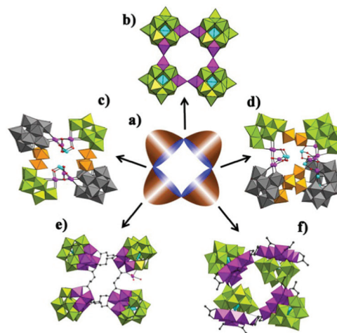
Fig. 13 (a) The schematic mode of rectangle TMSPTs. (b) View of [(\alpha-PW_{10}Fe_2O_{39})_4]^{7-} . (c) The structure of [Pd_{10}Se_{10}W_{52}O_{206}]^{40-} \{WO_6\} in tetravacant Dawson moieties: gray; \{WO_6\} in \{W_3O_{10}\} trimers: orange. (d) View of [Pd_{10}Se_{10}W_{52}O_{206}]^{40-} \{WO_6\} in tetravacant Dawson moieties: gray; \{WO_6\} in the \{W_2O_7\} dimer and the \{W_4O_{13}\} tetramer: orange. (e) The structure of [(A-\alpha-SiW_9O_{34})Ni_{14}(OH)_3]_4(OOC(CH_2)_3COO)_6]^{32-} . (f) The skeleton of [H_2Ni_{24}P_4W_{36}(OH)_{12}O_{136}(enMe)_{12}(CH_3COO)_4(H_2O)_{12}]^{2-} . \{WO_6\} : lime, \{XO_4\} : turquoise, TM, \{TMO_x\} and \{TMO_xN_y\} : light lavender, O: red, C: cray-80%, N: blue.
