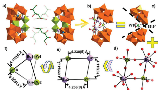
Fig. 3 (a) The combination of two [\text{Eu}_2(\text{H}_2\text{O})_2\text{W}_3\text{O}_6(\text{B}-\alpha\text{-TeW}_9\text{O}_{33})_2]^{4-} subunits and four \text{H}_2\text{glu}^{4-} linkers. (b) A dimeric [\text{Eu}_2(\text{H}_2\text{O})_2\text{W}_3\text{O}_6(\text{B}-\alpha\text{-TeW}_9\text{O}_{33})_2]^{4-} subunit containing W2, W6, Eu1 and Eu2 centers. (c) An openmouthed [\text{Te}_2\text{W}_{19}\text{O}_{68}]^{8-} segment containing a W18 bridge. (d) Top view of a tetra-nuclear [\text{Eu}_2(\text{H}_2\text{O})_2\text{W}_2\text{O}_4]^{10+} cluster constructed from W2, W6, Eu1 and Eu2 atoms. (e) A simplified view of the [\text{Eu}_2(\text{H}_2\text{O})_2\text{W}_2\text{O}_4]^{10+} cluster. (f) Side view of the simplified [\text{Eu}_2(\text{H}_2\text{O})_2\text{W}_3\text{O}_6]^{12+} cluster.
