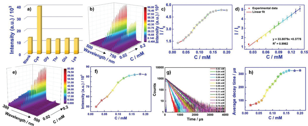
Fig. 11 (a) Change of the emission intensity at 614 nm of the Cu 2+ -quenching system based on 1 with addition of diverse aminoacids ( C_1 = 1.0 mg mL -1 , \lambda_{\text{ex}} = 394 nm). (b) Evolution of emission spectra of the Cu 2+ -quenching system based on 1 in different concentrations of Cys. (c) Variation of I/I_0 value of the emission intensity at 614 nm of the Cu 2+ -quenching system based on 1 with the concentration of Cys ( C_{\text{Cu}^{2+}} = 4.00 \times 10^{-2} mM) ( I is the emission intensity at 614 nm in different concentrations of Cys and I_0 is the emission intensity at 614 nm in the absence of Cys). (d) The linear variation of I/I_0 with the concentration of Cys ( C_{\text{Cu}^{2+}} = 4.00 \times 10^{-2} mM). (e) Evolution of excitation spectra of the Cu 2+ -quenching system based on 1 in different concentrations of Cys. (f) Change of the excitation intensity at 394 nm of the Cu 2+ -quenching system based on 1 in different concentrations of Cys. (g) Lifetime decay curves of the Cu 2+ -quenching system based on 1 in different concentrations of Cys. (h) Change of the average decay time ( \tau^* ) in different concentrations of Cys.
