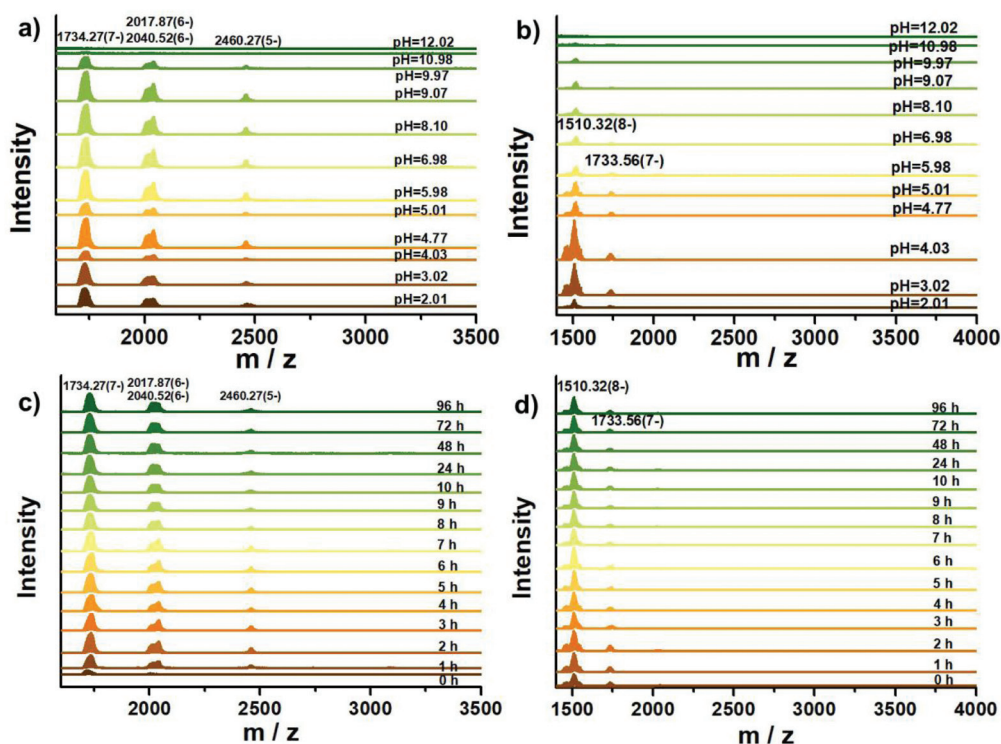
Fig. 7 (a) Enlarged view of the ESI-MS profiles in the range of 1600–3500 m/z of 1 in water at different pH values. (b) Evolution of the ESI-MS profiles of 1 in aqueous solution at different pH values. (c) Enlarged view of the ESI-MS profiles in the range of 1600–3500 m/z with time. (d) Evolution of the ESI-MS profiles of 1 with time in aqueous solution.
