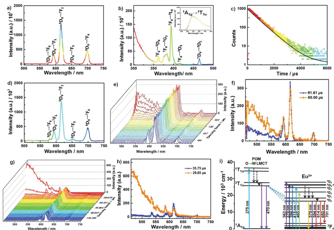
Fig. 5 (a) The solid-state emission spectrum of 1 under excitation at 394 nm. (b) The solid-state excitation spectrum of 1 taken by monitoring the strongest emission at 614 nm. (c) The solid-state lifetime decay curve of 1 obtained by monitoring the strongest emission at 614 nm. (d) The solid-state emission spectrum of 1 under excitation at 275 nm. (e) The TRES of 1 in the range of 80 to 200 \mu\text{s} under excitation at 394 nm. (f) The emission spectra of 1 at decay times of 80.00 and 91.61 \mu\text{s} under excitation at 394 nm. (g) The TRES of 1 in the range of 22.00 to 132.00 \mu\text{s} under excitation at 275 nm. (h) The emission spectra of 1 at the decay times of 29.85 and 35.75 \mu\text{s} under excitation at 275 nm. (i) The energy level diagram of 1 presenting the intramolecular energy transfer from TT fragments to \text{Eu}^{3+} ions.
