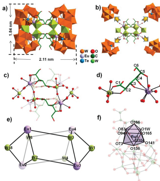
Fig. 1 (a) View of the tetrameric 1a POA. (b) Combination of four trivacant Keggin [B-α-TeW 9 O 33 ] 8- segments with a heterometallic 1b cluster. (c) View of the 1b cluster. (d) View of the [Eu 1 (H 2 O)W 3 (H 2 glu)O 2 ] + entity highlighting the flexible polyhydroxycarboxylic coordination mode of a H 2 glu 4- ligand. (e) Simplified view of the 1b cluster. (f) The distorted monocapped square antiprismatic geometry of the Eu 3+ ion.
