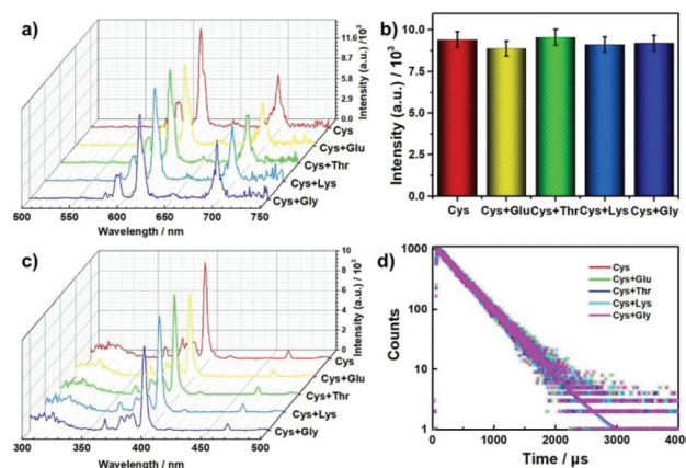
Fig. 12 (a) Changes in the emission spectra of the Cu 2+ -quenching system based on 1 (0.04 mM Cu 2+ cation) in the presence of both 0.10 mM of Cys and 0.10 mM of other amino acids. (b) Changes in the FL emission at 614 nm of the Cu 2+ -quenching system (0.04 mM of Cu 2+ ions) in the presence of both 0.10 mM of Cys and 0.10 mM of other amino acids. (c) Changes in the excitation spectra of the Cu 2+ -quenching system (0.04 mM of Cu 2+ ions) in the presence of both 0.10 mM of Cys and 0.10 mM of other amino acids. (d) Changes in the lifetime decay curves of the Cu 2+ -quenching system (0.04 mM of Cu 2+ ions) in the presence of both 0.10 mM of Cys and 0.10 mM of other amino acids.
