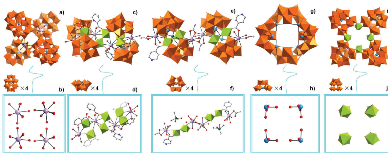
Fig. 2 (a–b) View of the tetrameric \{[\text{RE}(\text{H}_2\text{O})_5(\text{Te}^{\text{VI}}\text{W}_{18}\text{O}_{64})]_4\}^{44-} POA and the distribution of four RE bridges in it. 18 (c–d) View of the tetrameric [\text{Nd}_2(\text{H}_2\text{O})_4(\text{pica})_2\text{W}_2\text{O}_5][\{\text{Nd}(\text{H}_2\text{O})\text{W}_2(\text{Hpica})_2\text{O}_4\}(\text{B}-\beta\text{-TeW}_8\text{O}_{30}\text{H}_2)]^{24-} POA and the RE–TM heterometallic \{[\text{RE}_2(\text{H}_2\text{O})_4(\text{pica})_2\text{W}_2\text{O}_5][\{\text{RE}(\text{H}_2\text{O})\text{W}_2(\text{Hpica})_2\text{O}_4\}]_2\}^{20+} cluster in it. 7 (e–f) View of the tetrameric \{[\text{Sn}(\text{CH}_3)_2\text{W}_2\text{O}_4(\text{IN})][\{\text{B}-\alpha\text{-TeW}_8\text{O}_{31}\}\text{RE}(\text{H}_2\text{O})(\text{Ac})]_2\}^{20-} POA and the distribution of two [\text{Sn}(\text{CH}_3)_2]^{3+} groups and the inorganic–organic linear-shaped \{[\text{W}_2\text{O}_4(\text{IN})][\text{RE}(\text{H}_2\text{O})(\text{Ac})]_2\}^{14+} cluster in it. 8 (g–h) View of the tetrameric [\text{W}_{28}\text{Te}_8\text{O}_{112}]^{24-} POA and four \{\text{TeO}_4\} linkers in the square arrangement mode. 19a (i–j) View of the self-sorting cross-shaped tetrameric [\text{H}_4\text{P}_4\text{Te}_4\text{W}_{64}\text{O}_{224}]^{31-} POA and the distribution of the four \{\text{WO}_6\} linkers in it. 19b
