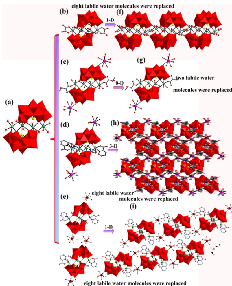
Figure 2. (a) View of the quadriFe III -inserted Krebs-type [Fe 4 (H 2 O) 10 (B-β-SbW 9 O 33 ) 2 ] 10- unit. (b) View of the ox-substituted Krebs-type [Fe 4 (ox) 4 (B-β-SbW 9 O 33 ) 2 ] 14- unit. (c) View of the thr-substituted structure of [Ln(H 2 O) 8 ] 2 [Fe 4 (H 2 O) 8 (thr) 2 ][B-β-SbW 9 O 33 ] 2 ·22H 2 O. (d) View of the pic-substituted Krebs-type unit observed in 1–5 in this paper. (e) View of the pic-substituted Krebs-type unit observed in 8–9 in this paper. (f) One-D chain formed by ox-substituted Krebs-type units. (g) thr-substituted isolated structure. (h) Three-D extended framework observed in 1–5 in this paper. (i) One-D double chain observed in 8–9 in this paper.
