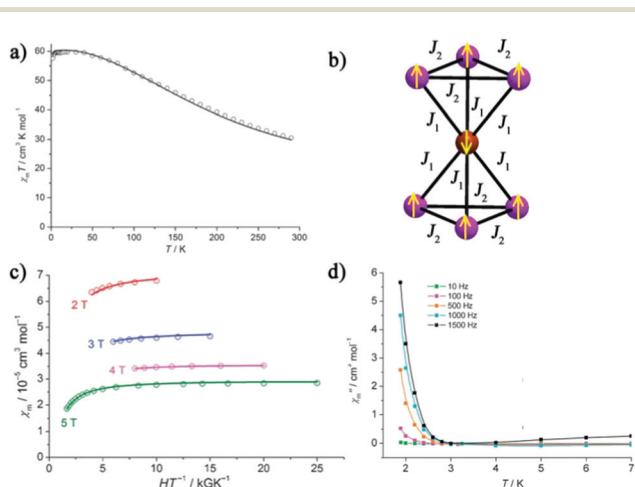
Fig. 19 (a) Temperature dependence of \chi_m T for [(\alpha\text{-P}_2\text{W}_{15}\text{O}_{56})_2\text{Mn}_6^{\text{III}}\text{Mn}^{\text{IV}}\text{O}_6(\text{H}_2\text{O})_6]^{14-} . (b) The magnetic exchange model and the ground state spin alignments of the \{\text{Mn}_6^{\text{III}}\text{Mn}^{\text{IV}}\text{O}_8\} core. (c) The field-dependence of \chi_m at low temperatures for [(\alpha\text{-P}_2\text{W}_{15}\text{O}_{56})_2\text{Mn}_6^{\text{III}}\text{Mn}^{\text{IV}}\text{O}_6(\text{H}_2\text{O})_6]^{14-} . (d) Temperature dependence of the out-of-phase susceptibility \chi''_m ( H_{\text{dc}} = 0 ). [Copied from ref. 18d]. Reprinted with permission from ref. 18d. Copyright The Royal Society of Chemistry 2012.
