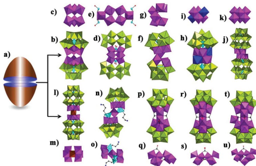
Fig. 4 (a) The schematic mode of embedded-sandwich-type TMSPTs. (b, c) View of [\text{Fe}_6(\text{OH})_3(\text{A}\text{-}\alpha\text{-GeW}_9\text{O}_{34}(\text{OH})_3)_2]^{11-} and its trigonal prismatic core \{\text{Fe}_6(\text{OH})_3\} . (d, e) View of [\text{Fe}_6\text{Se}_6\text{W}_{34}\text{O}_{124}(\text{OH})_{16}]^{18-} and its central core \{\text{Fe}_6\text{W}_6\} . (f, g) View of [(\text{Ni}_6(\text{H}_2\text{O})_4(\mu_2\text{-H}_2\text{O})_4(\mu_3\text{-OH})_2)(\text{SiW}_9\text{O}_{34})_2]^{10-} and its central core \{\text{Ni}_6(\text{H}_2\text{O})_4(\mu_2\text{-H}_2\text{O})_4(\mu_3\text{-OH})_2\} . (h, i) View of [(\text{B}\text{-}\alpha\text{-GeW}_9\text{O}_{34})_2\{\text{Mn}_4^{\text{III}}\text{Mn}_2^{\text{IV}}\text{O}_4(\text{H}_2\text{O})_4\}]^{12-} and its mixed-valence double-cubane core \{\text{Mn}_4^{\text{III}}(\text{H}_2\text{O})_2\text{Mn}_2^{\text{IV}}\text{O}_4(\text{H}_2\text{O})_2\} [ \text{Mn}^{\text{III}} : blue]. (j) View of the POA in [\text{P}_4\text{V}_6\text{W}_{30}\text{O}_{120}]^{10-} . (k) The double-cubane \{\text{V}_6\text{O}_8\} core in [\text{P}_4\text{V}_6\text{W}_{30}\text{O}_{120}]^{10-} . (l, m) View of [(\alpha\text{-P}_2\text{W}_{15}\text{O}_{56})_2\text{Mn}_6^{\text{III}}\text{Mn}^{\text{IV}}\text{O}_6(\text{H}_2\text{O})_6]^{14-} and its double-cubane core \{\text{Mn}_6^{\text{III}}\text{Mn}^{\text{IV}}\text{O}_8\} [ \text{Mn}^{\text{IV}} : brown]. (n, o) View of [(\text{B}\text{-}\alpha\text{-PW}_9\text{O}_{34})\text{Co}_3(\text{OH})(\text{H}_2\text{O})_2(\text{Ale})_2\text{Co}]^{14-} and its \text{Co}_7 -core [P: turquoise]. (p, q) View of [\text{Ni}_7(\text{OH})_4(\text{H}_2\text{O})(\text{CO}_3)_2(\text{HCO}_3)(\text{A}\text{-}\alpha\text{-SiW}_9\text{O}_{34})(\beta\text{-SiW}_{10}\text{O}_{37})]^{10-} and its central core \{\text{Ni}_7(\text{OH})_4(\text{H}_2\text{O})(\text{CO}_3)_2(\text{HCO}_3)\} . (r, s) View of [(\text{A}\text{-}\alpha\text{-SiW}_9\text{O}_{34})_2\text{Co}_8(\text{OH})_6(\text{H}_2\text{O})_2(\text{CO}_3)_3]^{16-} and its central core \{\text{Co}_8(\text{OH})_6(\text{H}_2\text{O})_2(\text{CO}_3)_3\} . (t, u) View of [(\text{A}\text{-}\alpha\text{-SiW}_9\text{O}_{34})_2\text{Ni}_9(\text{OH})_6(\text{H}_2\text{O})_6(\text{CO}_3)_3]^{14-} and its central core \{\text{Ni}_9(\text{OH})_6(\text{H}_2\text{O})_6(\text{CO}_3)_3\} . \{\text{WO}_6\} : lime, \{\text{XO}_4\} : turquoise, TM and \{\text{TMO}_x\} : light lavender, O: red, C: cray-80%, N: blue.
