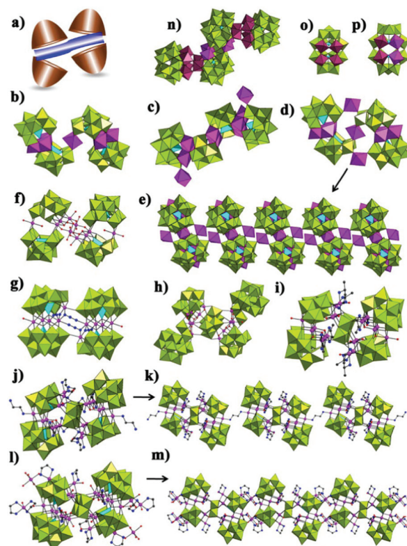
Fig. 9 (a) The schematic mode of “S”-shaped TMSPTs. (b) View of [(\beta\text{-}\beta\text{-SiW}_9\text{O}_{33}(\text{OH}))(\beta\text{-}\beta\text{-SiW}_8\text{O}_{29}(\text{OH})_2)\text{Co}_3(\text{H}_2\text{O})_2]_2\text{Co}(\text{H}_2\text{O})_2]^{20-} . (c) View of [\text{Mn}_2^{\text{II}}(\text{Mn}^{\text{III}}(\text{H}_2\text{O})_5\text{Mn}^{\text{III}}(\text{H}_2\text{O})(\beta\text{-}\beta\text{-SiW}_9\text{O}_{34})(\beta\text{-}\beta\text{-SiW}_6\text{O}_{26}))_2]^{18-} . (d, e) View of [\{\text{Mn}(\text{H}_2\text{O})_3\}_2[\text{Mn}(\text{H}_2\text{O})_2][(\beta\text{-}\beta\text{-SiW}_9\text{O}_{33}(\text{OH}))\text{Mn}_3(\text{H}_2\text{O})(\beta\text{-}\beta\text{-SiW}_8\text{O}_{30}(\text{OH}))]_2]^{18-} and its 1-D chain. (f) View of [(\text{Fe}(\text{H}_2\text{O})_2)(\text{SiW}_{10}\text{O}_{35})(\text{SiFe}_2\text{W}_8\text{O}_{35})_2(\text{Fe}_4\text{O}_4(\text{H}_2\text{O})_6)]^{26-} . (g) View of [\text{Cu}_{10}(\text{H}_2\text{O})_2(\text{N}_3)_4(\text{GeW}_9\text{O}_{34})_2(\text{GeW}_8\text{O}_{31})_2]^{24-} . (h) View of [\{\text{Mn}^{\text{III}}(\text{Mn}^{\text{II}}(\text{H}_2\text{O})_5\text{Mn}^{\text{III}}(\text{H}_2\text{O})(\beta\text{-}\beta\text{-SiW}_9\text{O}_{34})(\beta\text{-}\beta\text{-SiW}_6\text{O}_{26}))_2(\text{W}_6\text{O}_{22})(\text{H}_2\text{W}_8\text{O}_{32})(\text{H}_4\text{W}_{13}\text{O}_{46})_2\}]^{26-} . (i) View of [\text{H}_6\text{Ni}_{20}\text{P}_4\text{W}_{34}(\text{OH})_4(\text{O}_{136}(\text{en})\text{Me})_8(\text{H}_2\text{O})_6]^{6-} . (j, k) View of [\text{H}_8\text{Ni}_{20}\text{P}_4\text{W}_{34}(\text{OH})_4(\text{O}_{136}(\text{en})_9)(\text{H}_2\text{O})_4]^{4-} and its 1-D chain. (l, m) View of [\{(\alpha\text{-AsW}_6\text{O}_{26})\text{Ni}_6(\text{OH})_2(\text{H}_2\text{O})_3(\text{en})(\beta\text{-}\alpha\text{-AsW}_9\text{O}_{34})\}_2[\text{W}_4\text{O}_{16}][\text{Ni}_3(\text{H}_2\text{O})_2(\text{en})]_2]^{16-} and its 1-D chain. (n, o, p) View of [\text{Fe}_{10}\text{Se}_8\text{W}_{62}\text{O}_{222}(\text{OH})_{18}(\text{H}_2\text{O})_4]^{28-} and two saturated \{\alpha\text{-Se}_2\text{W}_{16}\text{Fe}_2\} and \{\gamma\text{-Se}_2\text{W}_{15}\text{Fe}_3\} fragments [W/Fe: violet]. [\text{WO}_6] : lime, \{\text{XO}_4\} : turquoise, TM and \{\text{TM}_x\} : light lavender, O: red, C: cray-80%, N: blue].
