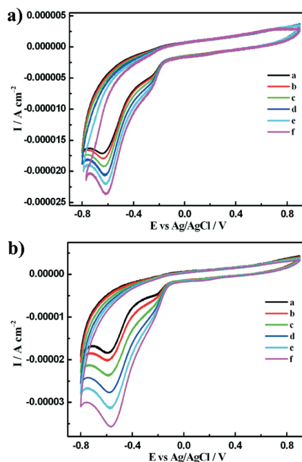
Fig. 9 (a) Cyclic voltammograms of 1 (concentration: 1.73 \times 10^{-4} mol L ^{-1} ) in 0.5 mol L ^{-1} Na _2 SO _4 + H _2 SO _4 aqueous solution, pH = 1.44, with the addition of various concentrations of NaNO _2 (a: 0, b: 1 \times 10^{-5} , c: 3 \times 10^{-5} , d: 7 \times 10^{-5} , e: 1 \times 10^{-4} , f: 1.5 \times 10^{-4} mol L ^{-1} ). (b) Cyclic voltammograms of 1 (concentration: 1.73 \times 10^{-4} mol L ^{-1} ) in 0.5 mol L ^{-1} Na _2 SO _4 + H _2 SO _4 aqueous solution, pH = 1.44, with the addition of various concentrations of NaBrO _3 (a: 0, b: 1 \times 10^{-5} , c: 3 \times 10^{-5} , d: 5 \times 10^{-5} , e: 7 \times 10^{-5} , f: 9 \times 10^{-5} mol L ^{-1} ).
